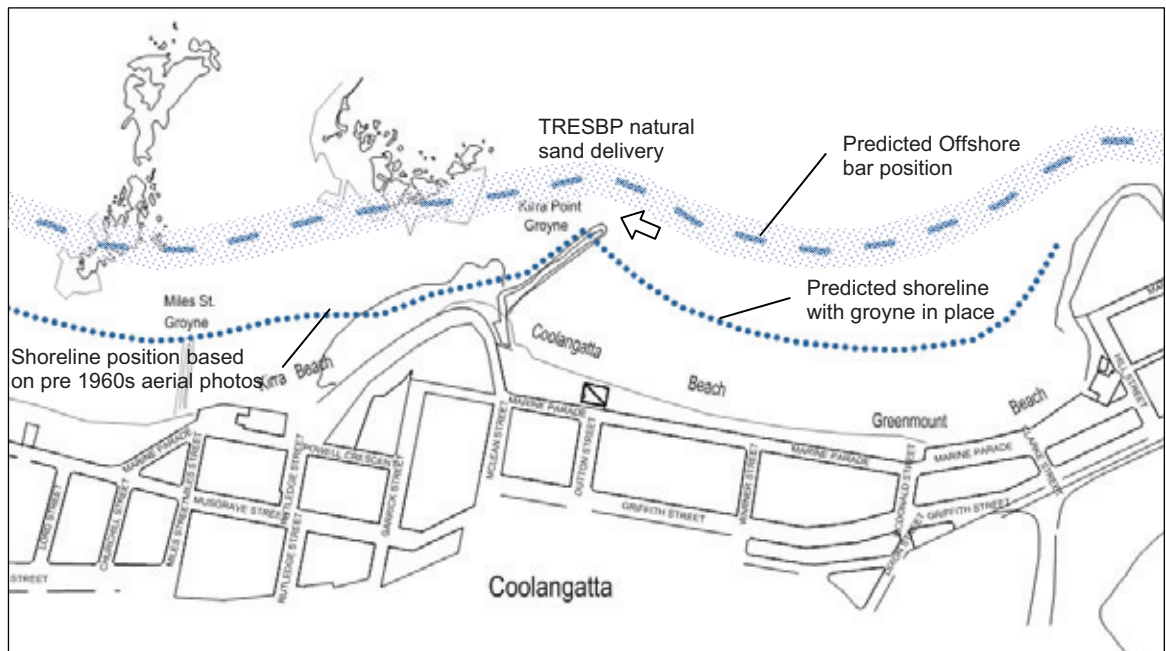
Figure 24 Post-TRESBP including Kirra Point groyne (natural sand supply)
