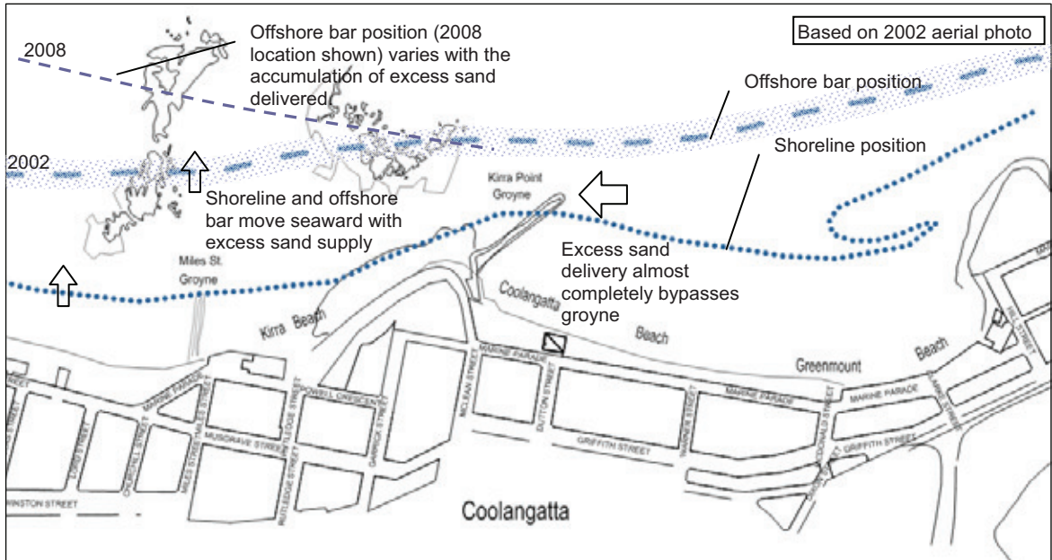
Figure 23 Post-TRESBP including Kirra Point groyne (excess sand supply)
